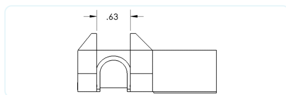
3rd Gen. Tip Pocket Part# 15-02949
