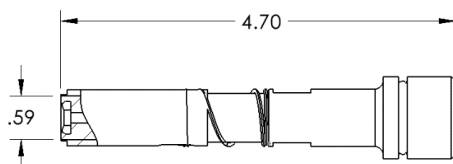
.59 Dia Vacuum Tip Holder Part# 15-03047
