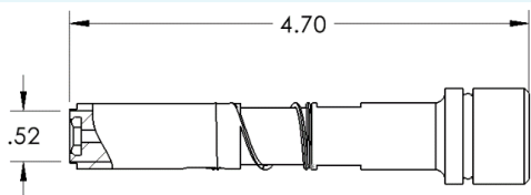
.52 Dia Vacuum Tip Holder Part# 15-03042
