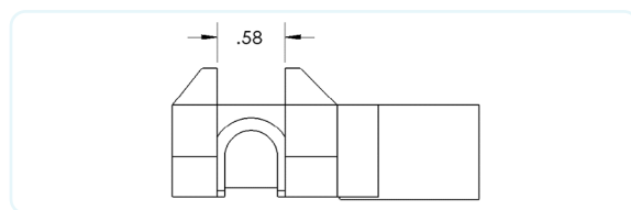
2nd Gen. Tip Pocket Part# 15-02237
