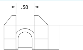
2nd Gen. Tip Pocket Part# 15-02237
