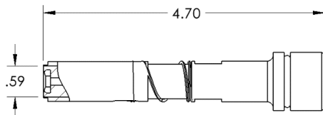
.59 Dia Vacuum Tip Holder Part# 15-03047
